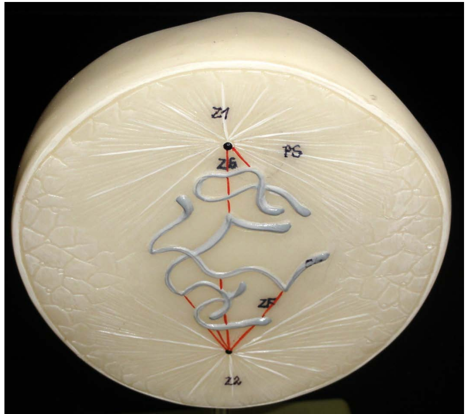
Prophase Late
