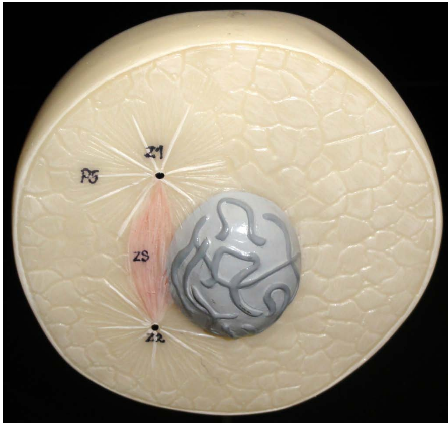
Prophase Early
