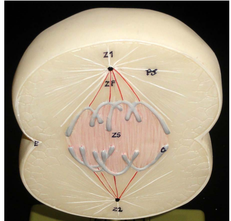
Late Anaphase
